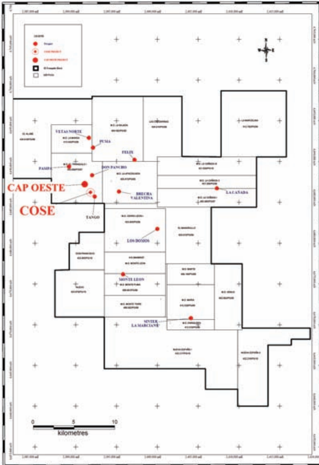
Figure 4-2 Location of the COSE Project in relation to Cap Oeste and the El Tranquilo I MD Claim
