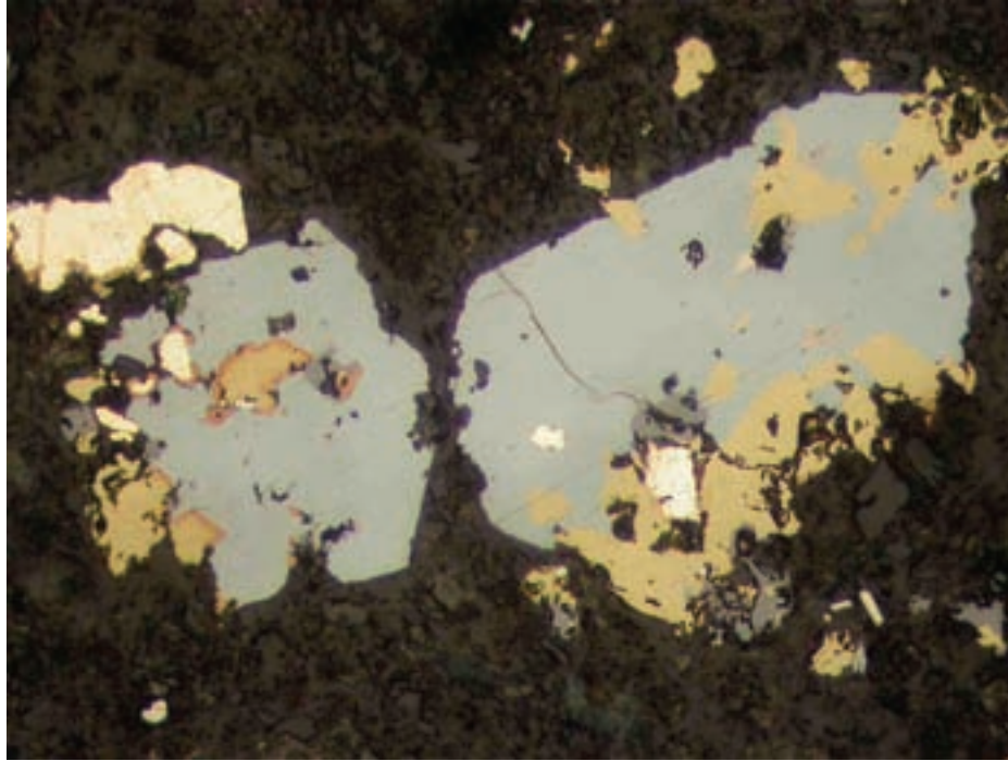
Figure 7-13 DDH CSE-13 (209.7m). Composite aggregates of proustite-pyrargyrite (pale blue-grey) and chalcopyrite (yellow), with bright creamy grains of gold-electrum in illite-sericite-quartz gangue.
