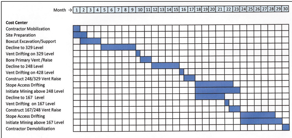
Figure 16-1 COSE Project – Development/Mining Schedule
