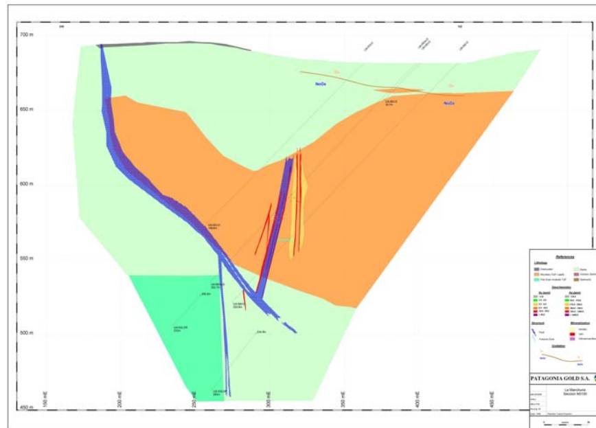
Figure 10.2 Cross-Section N5100
