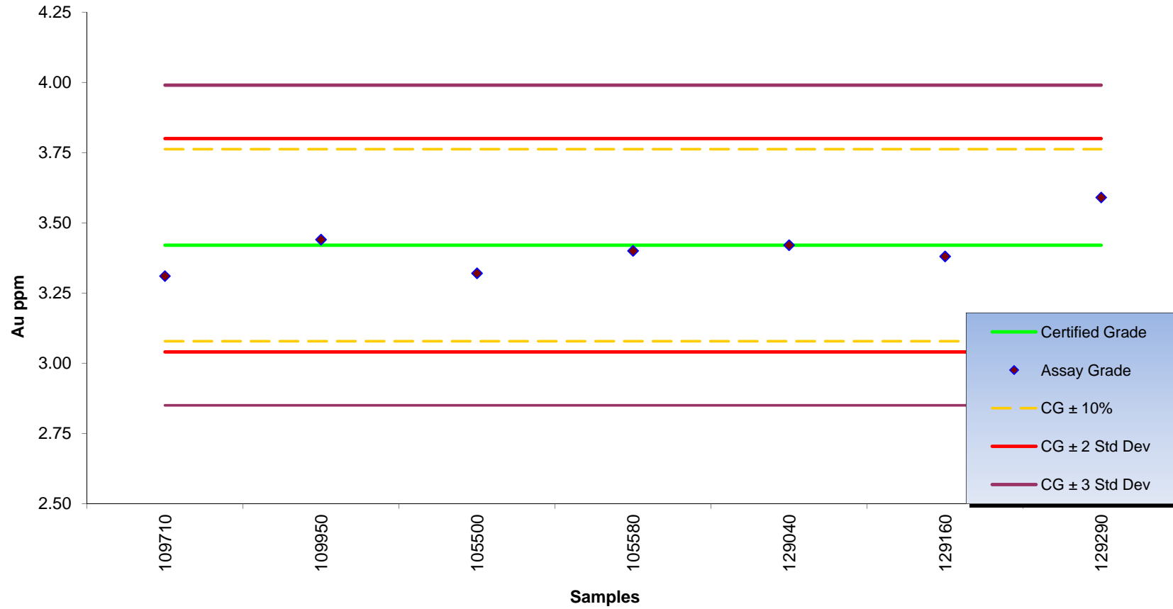
Control Chart for PGSA Certified Reference Standard G999-8 Holes LM-077-D to LM-095-D
