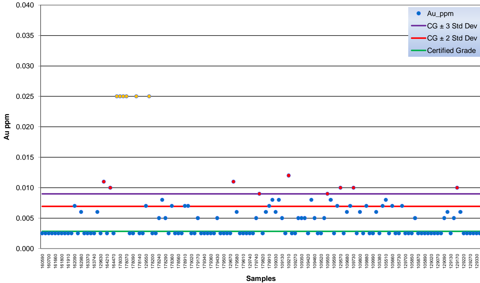
Control Chart for PGSA Certified Reference Blank Grey Blank Holes LM-004-D to LM-095-D
